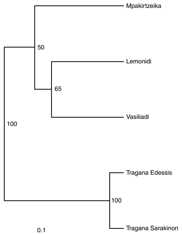
Fig. 2. Unweighted pair group method with arithmetic mean dendrogram showing similarities among five Prunus avium cultivars based on 11 simple sequence repeat loci. Numbers below branches represent bootstrapping values.
