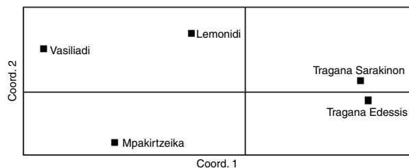
Fig. 3. Scatter plot of the first and second PCoA of the Prunus avium cultivars studied.
